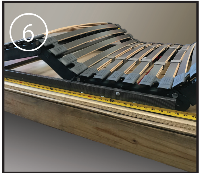
Side Profile Showing Length from Foot to Hinge Position About 44.5 Inch (Customizable)
